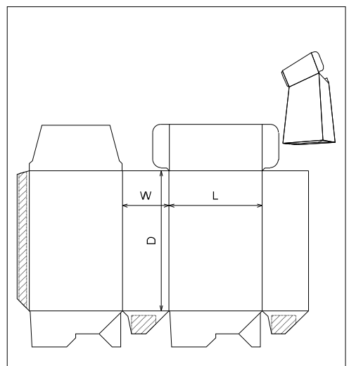
ECMA Folding Carton\Group A\ECMA A6040 - FC0116 - Side Tuck Crash Lock Base
