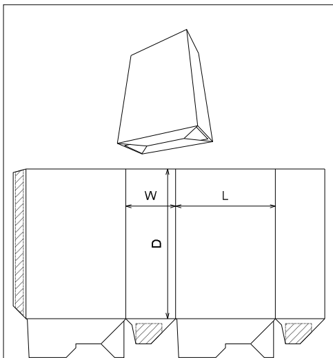
ECMA Folding Carton\Group A\ECMA A6001 - FC0125 - Open Ended Crash Lock Base
