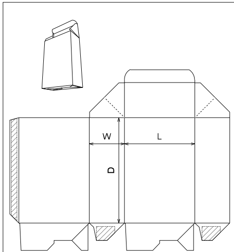
ECMA Folding Carton\Group A\ECMA A6099 - FC0107 - Webbed Tuck Crash Lock Base
