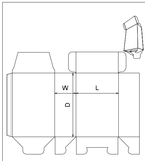
ECMA Folding Carton\Group A\ECMA A5540 - FC0118 - Side Tuck Snap Lock Base
