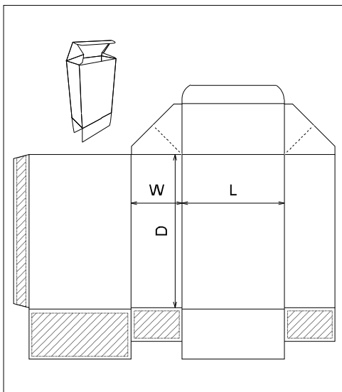
ECMA Folding Carton\Group A\ECMA A1099 - FC1211 - Webbed Tuck Square Flap Skillet
