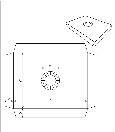
ECMA Folding Carton\Group F\ECMA F8003 - FC0617 - 4 Sided Platform with Centre Hole
