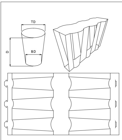
ECMA Folding Carton\Group E\ECMA E1021 - FC0404 - Non-Glued Wrap
