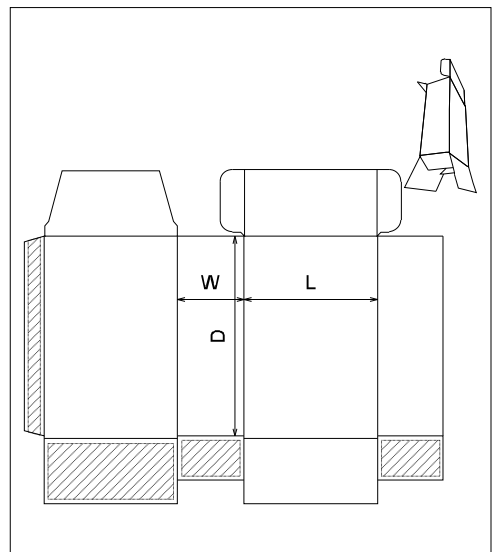
ECMA Folding Carton\Group A\ECMA A1040 - FC0213 - Side Tuck Square Flap Skillet
