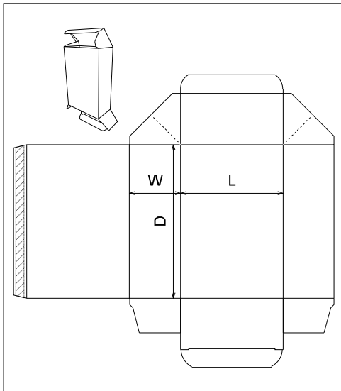
ECMA Folding Carton\Group A\ECMA A2099 - FC0222 - Webbed Tuck Tuck to Back
