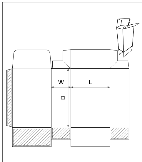
ECMA Folding Carton\Group A\ECMA A1045 - FC0212 - Sieve Proof Square Flap Skillet
