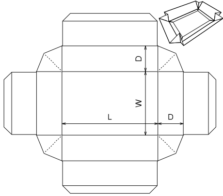
ECMA Folding Carton\Group B\ECMA B1011 - FC0303 - Webbed Self Locking Tray
