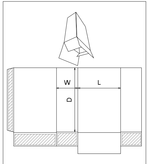
ECMA Folding Carton\Group A\ECMA A1101 - Open Ended Reduced Flap Skillet
