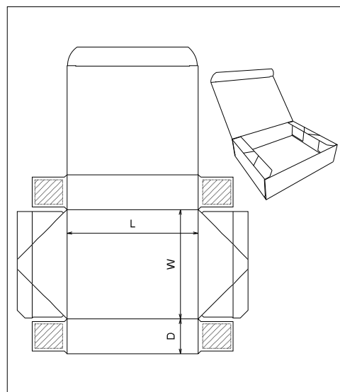
ECMA Folding Carton\Group B\ECMA B4050 - FC0308 - Four Corner Hinged Lid
